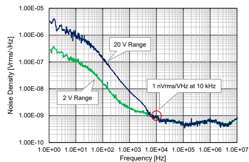
Figure 5. HC-ULNF and ULNF provide excellent noise density performance
