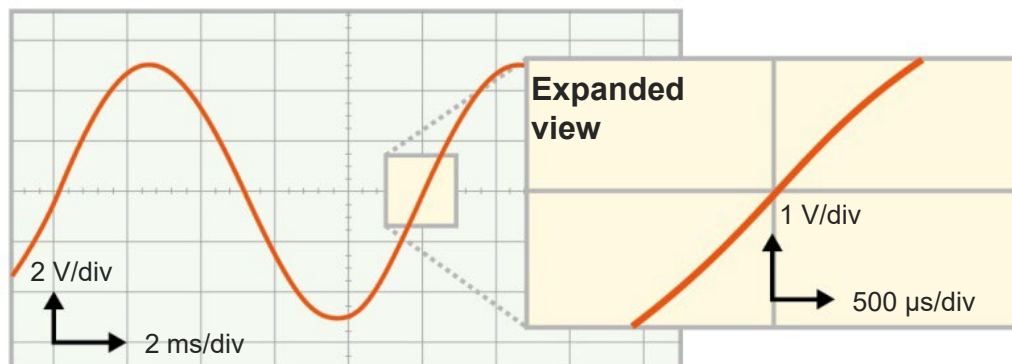
Figure 12. Sinusoid waveform comparison at 100 Hz (B2961C/B2962C)
