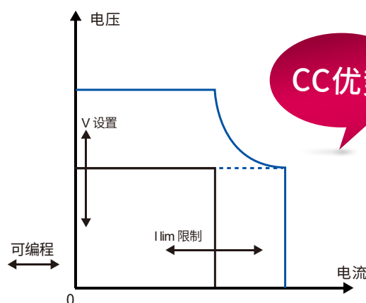
电池充放电高速无缝, 无过冲切换 (CV-High, CC-High, CC优势)
