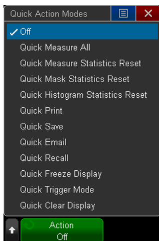
Figure 55. QuickAction menu.
