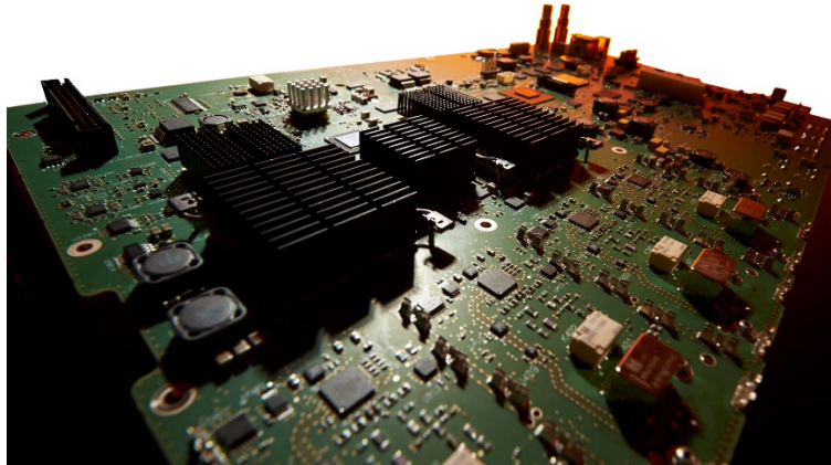
Figure 5. The new 6-GHz front-end design.
